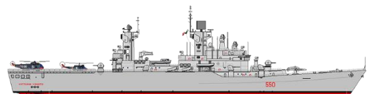
Vittorio Veneto helicopter cruiser class
